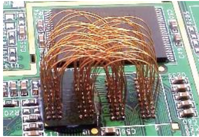
BGA Fly Line
